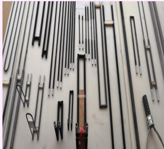
SiC and Silicon molybdenum rod
